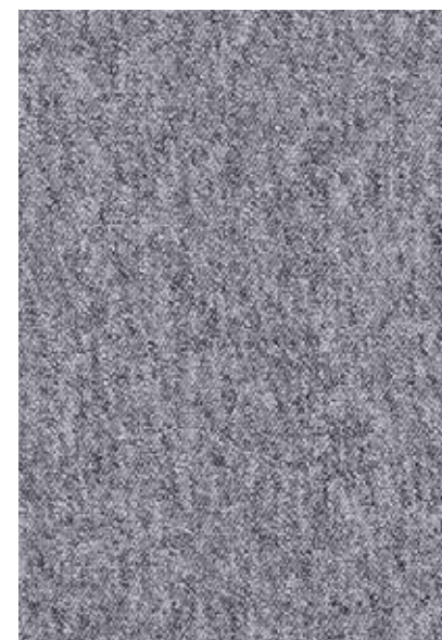
Snowstorm
