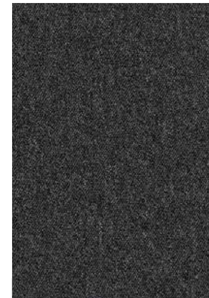
Monsoon
